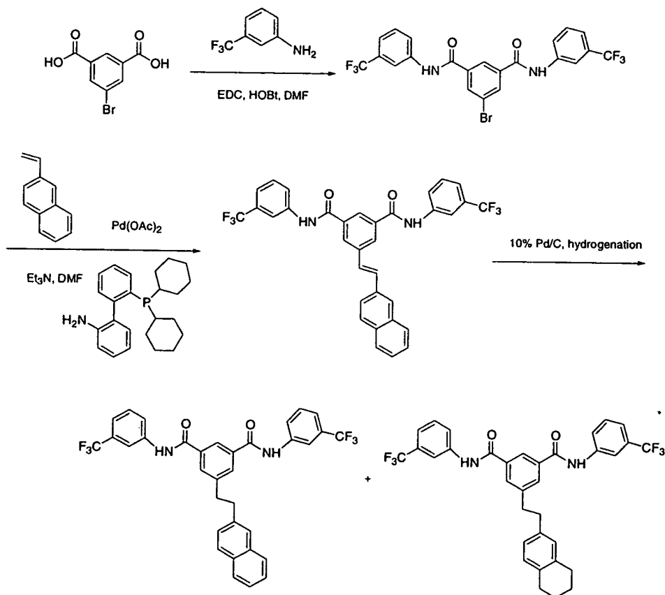
Scheme I-F
